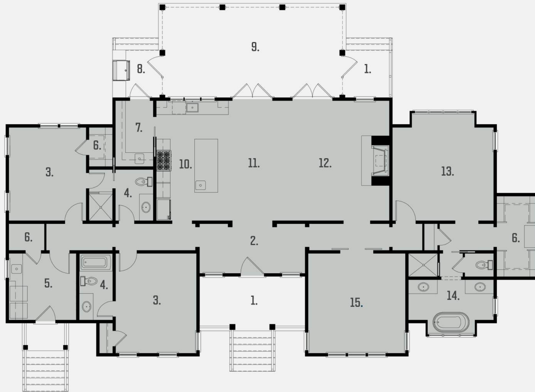
FIRST FLOOR
